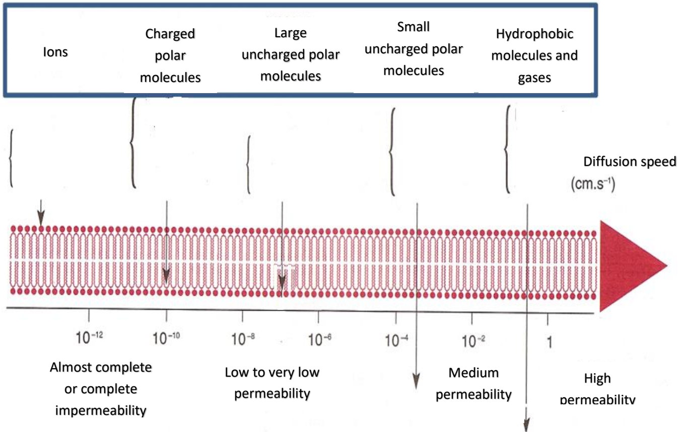
Figure 1. Permeability of the lipid bilayer
