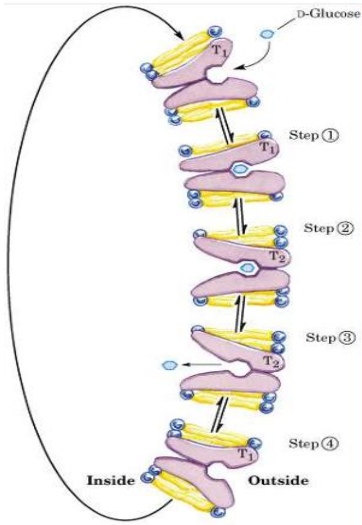
Figure 3. Structure and operating model of a glucose permease.
