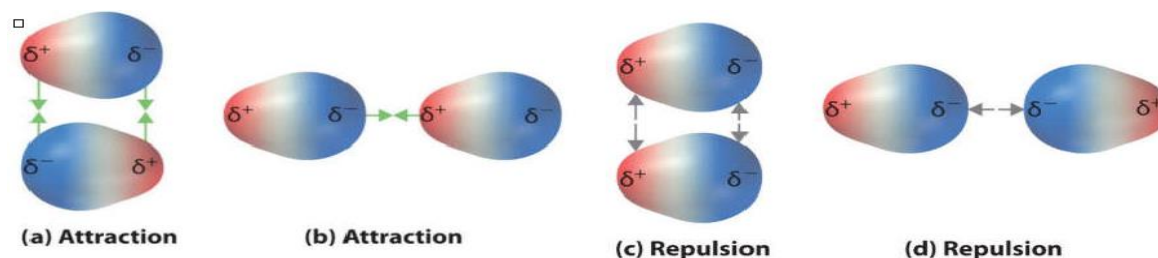
Fig . dipole-dipole interaction
